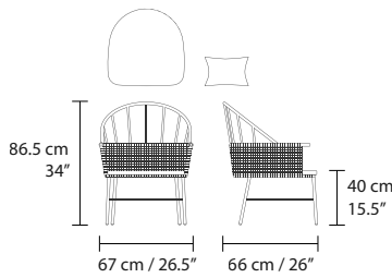
LOUNGE CHAIR 12.5 kg / 27.5 lb
