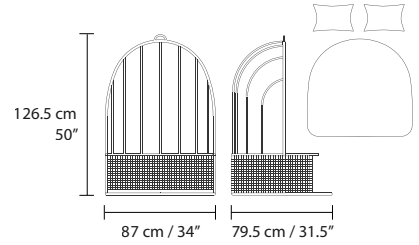
HANGING CHAIR 13.5 kg / 29.5 lb
