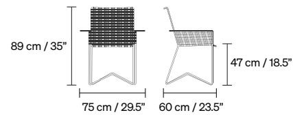
PORSET SILLA DINING CHAIR 13 kg / 28 lb
