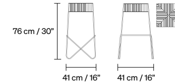
ROSARITO BAR STOOL 7 kg / 15.5 lb
