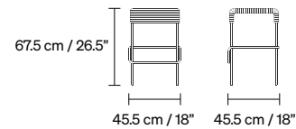
CALIFORNIA COUNTER STOOL 8.5 kg / 19 lb
