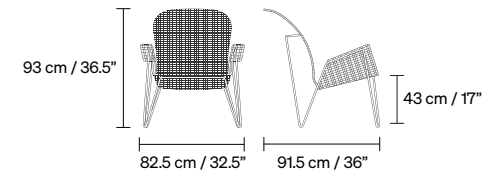
PORSET SILLA ALTA LOUNGE CHAIR 15 kg / 33.5 lb
