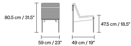
CALIFORNIA DINING CHAIR 6.5 kg / 14.5 lb
