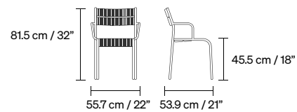
EKOL DINING ARMCHAIR 7.2 kg / 16 lb
