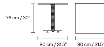
BARCELONETTE SQUARE DINING TABLE 26 kg / 57 lb
