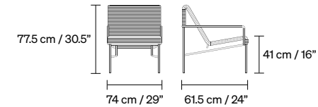
CALIFORNIA LOUNGE CHAIR 12 kg / 26.5 lb
