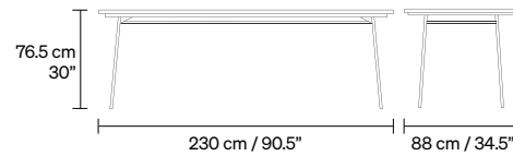
1730 RECTANGLE TABLE L 50 kg / 110.5 lb
