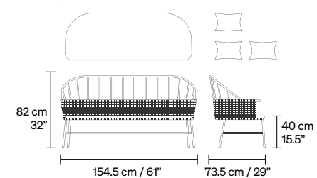
1730 LOVESEAT 23.5 kg / 51.5 lb
