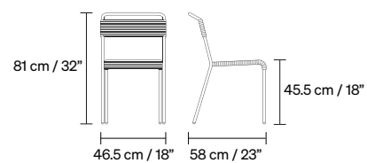
COLORÍN DINING CHAIR 5.5 kg / 12 lb
