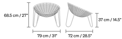
TODOS SANTOS LOUNGE CHAIR 10 kg / 22 lb
