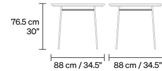
1730 SQUARE DINING TABLE 24 kg / 53 lb
