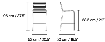
BARCELONETTE COUNTER STOOL 8 kg / 18 lb
