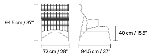
TABACHÍN LOUNGE CHAIR 20.5 kg / 45 lb
