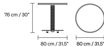
BARCELONETTE DINING ROUND TABLE 25 kg / 55 lb
