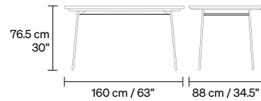
1730 RECTANGLE TABLE M 36.5 kg / 81 lb
