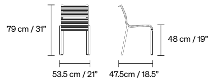
BARCELONETTE DINING CHAIR 6.5 kg / 14.5 lb
